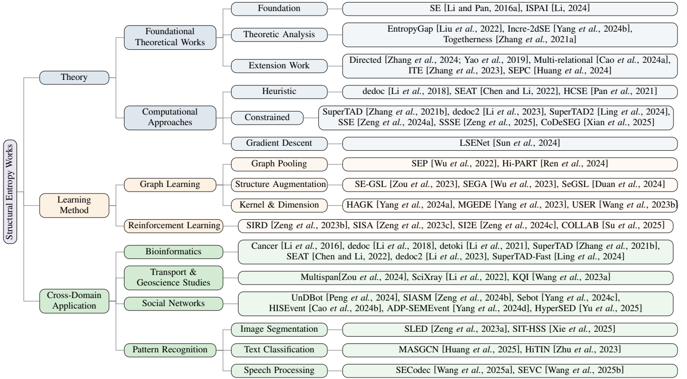
Figure 1: A taxonomy of Structural Entropy works.
