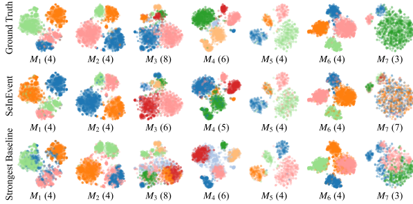
Figure 6: (RQ4) Comparison of SeInEvent clustering results with actual results and the strongest baseline. The number of clusters is indicated in parentheses.
