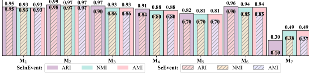
Figure 4: (RQ2) Results of experiments about incremental learning analysis. SeEvent is a degenerate model of SeInEvent, i.e., no incremental learning is performed and only the initial message block M_0 is used for training.
