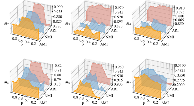
Figure 5: (RQ3) Results of hyperparameter sensitivity.
