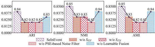
Figure 3: (RQ2) Results of ablation experiments. Values are the average of all message blocks.
