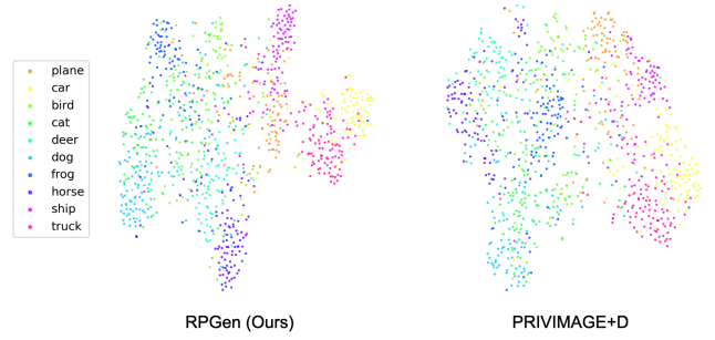
Figure 1: t-SNE visualization of feature embeddings from synthetic CIFAR-10 images generated by RPGen (left) and PRIVIMAGE+D (right).
